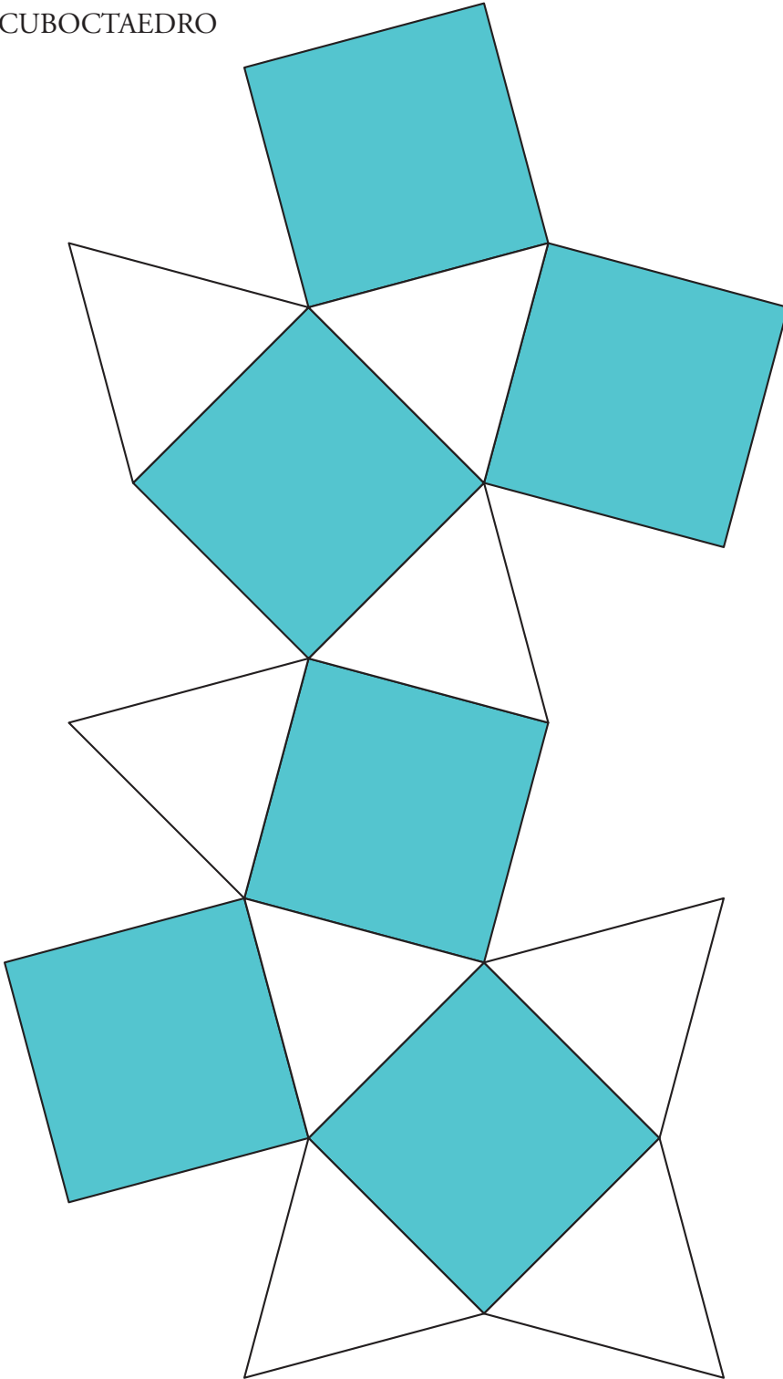
OCTAEDRO - CUBOCTAEDRO
